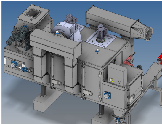
Design drawing of the Pilot Belt Dryer BD 750/2
